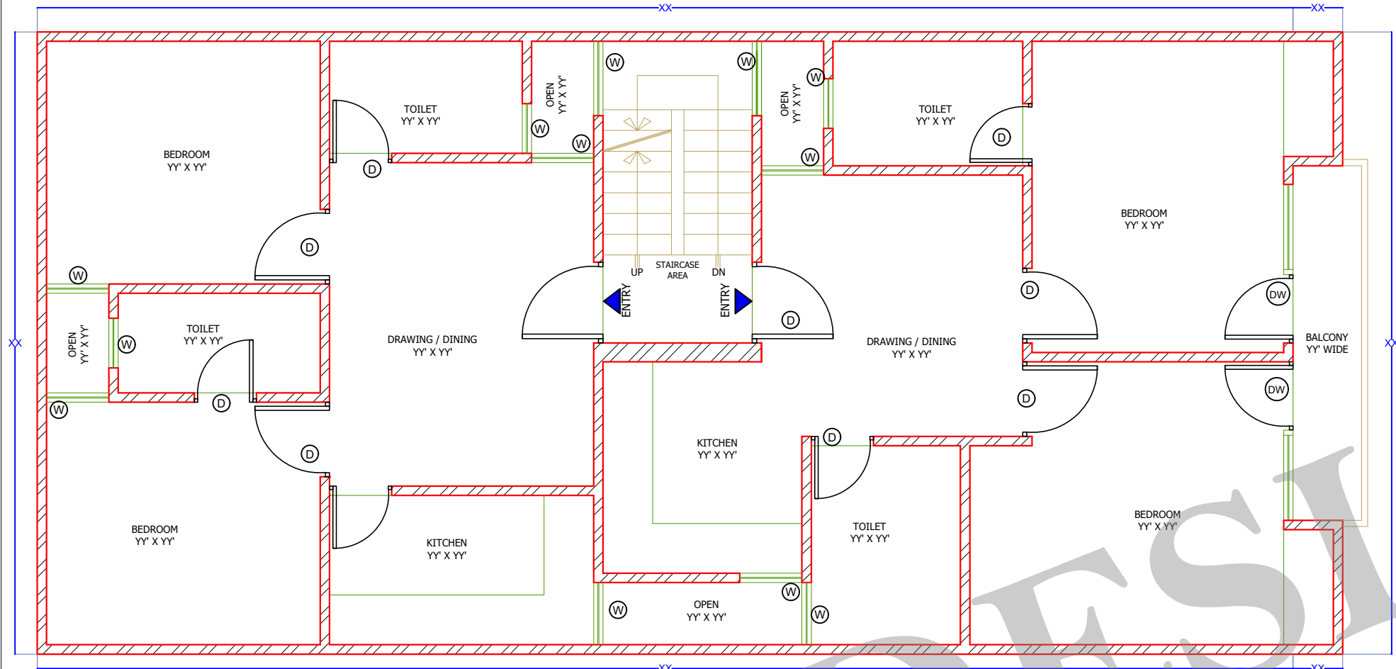
TYPICAL FLOOR PLAN NOT TO SCALE
